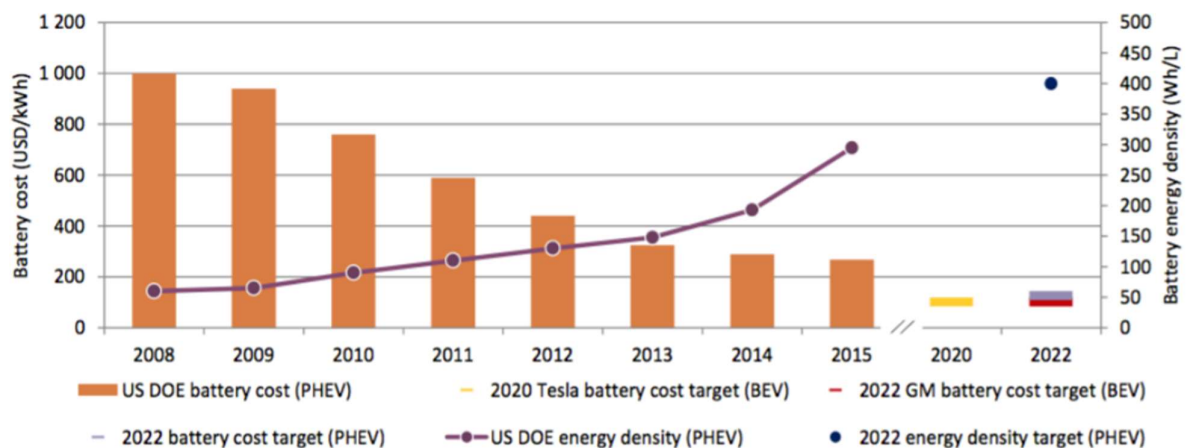
Figure 7. Battery production cost per kWh and energy density over time. 16
