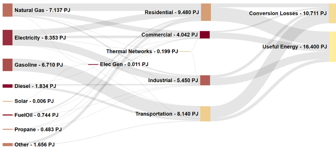
Figure 11. BAU Sankey diagram of energy sources, uses, and use/losses, 2050.
